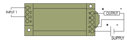
CR4520 Single Phase - 4 - 20 mADC Output
