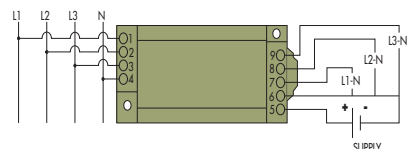
CR4570 3 Phase, 4 Wire - 0 - 5 VDC Output
