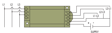
CR4550 3 Phase, 3 Wire - 0 - 5 VDC Output
