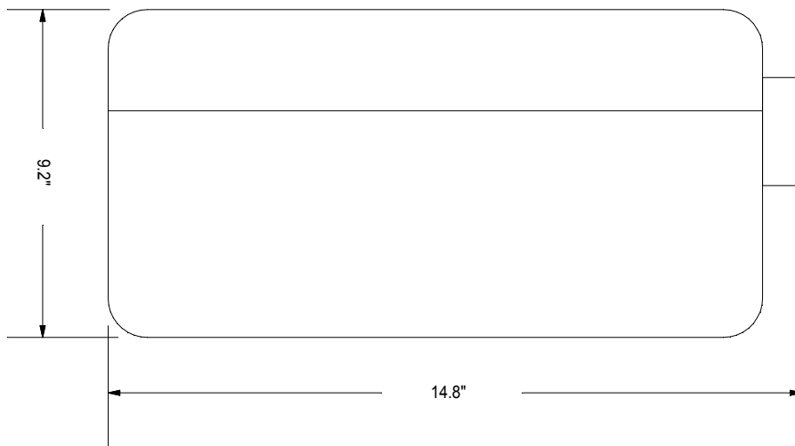
Enc350 Enclosure Outside Dimensions Shown with optional Surface Mounting Bracket (drawing is not to scale)
