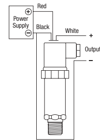
VOLTAGE, 3-WIRE
